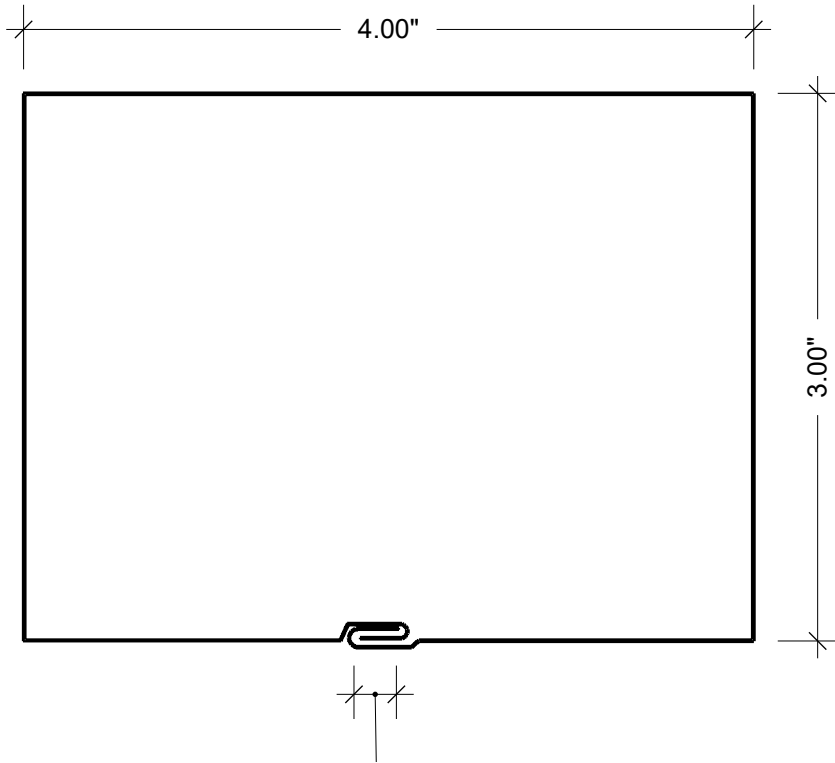
0.33" Closed Double Seam Acme Lock
